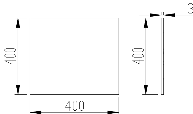
( figure 4 ) Aluminum Radiator Size
